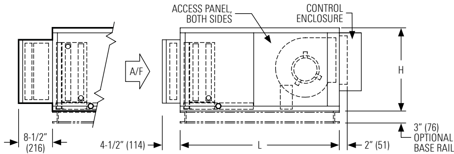
HIGH EFFICIENCY FILTER RACK SIDE VIEW
